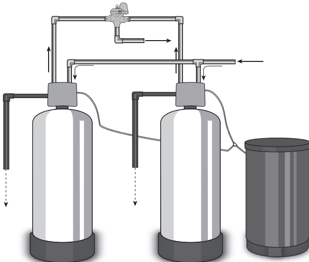
1" – 1.25" TWIN ALT
