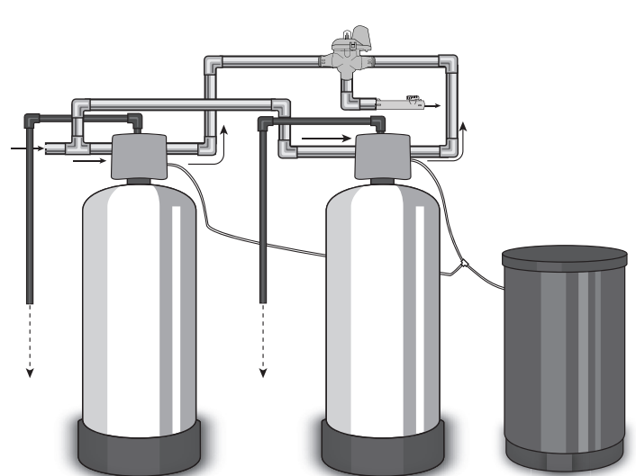
1.5" – 2.0" TWIN
